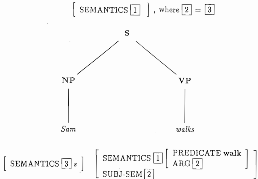
Figure 1: A sketch of the semantic derivation of Sam walks , \text{walk}(s) as this would proceed using unification. Unification applies to syntactic and semantic representations alike, eliminating the need to compute these in distinct processes, and unification is employed to bind variables to argument positions, eliminating the need for (a great deal of) \beta -reduction as used in schemes derived from Montague and the lambda calculus.
