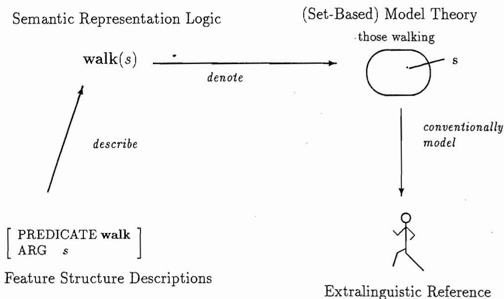
Figure 2: The relation of feature-based semantics to semantic representation logic, model theory, and the extralinguistic objects of discourse. A simpler, but ultimately unsatisfactory view, would eliminate the semantic representation logic.
